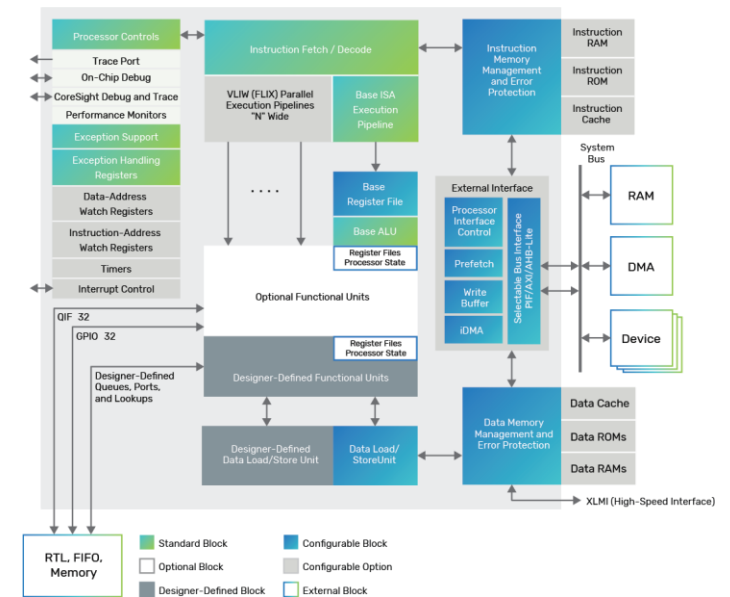
Block diagram of Xtensa LX7 processor architecture ( source )
